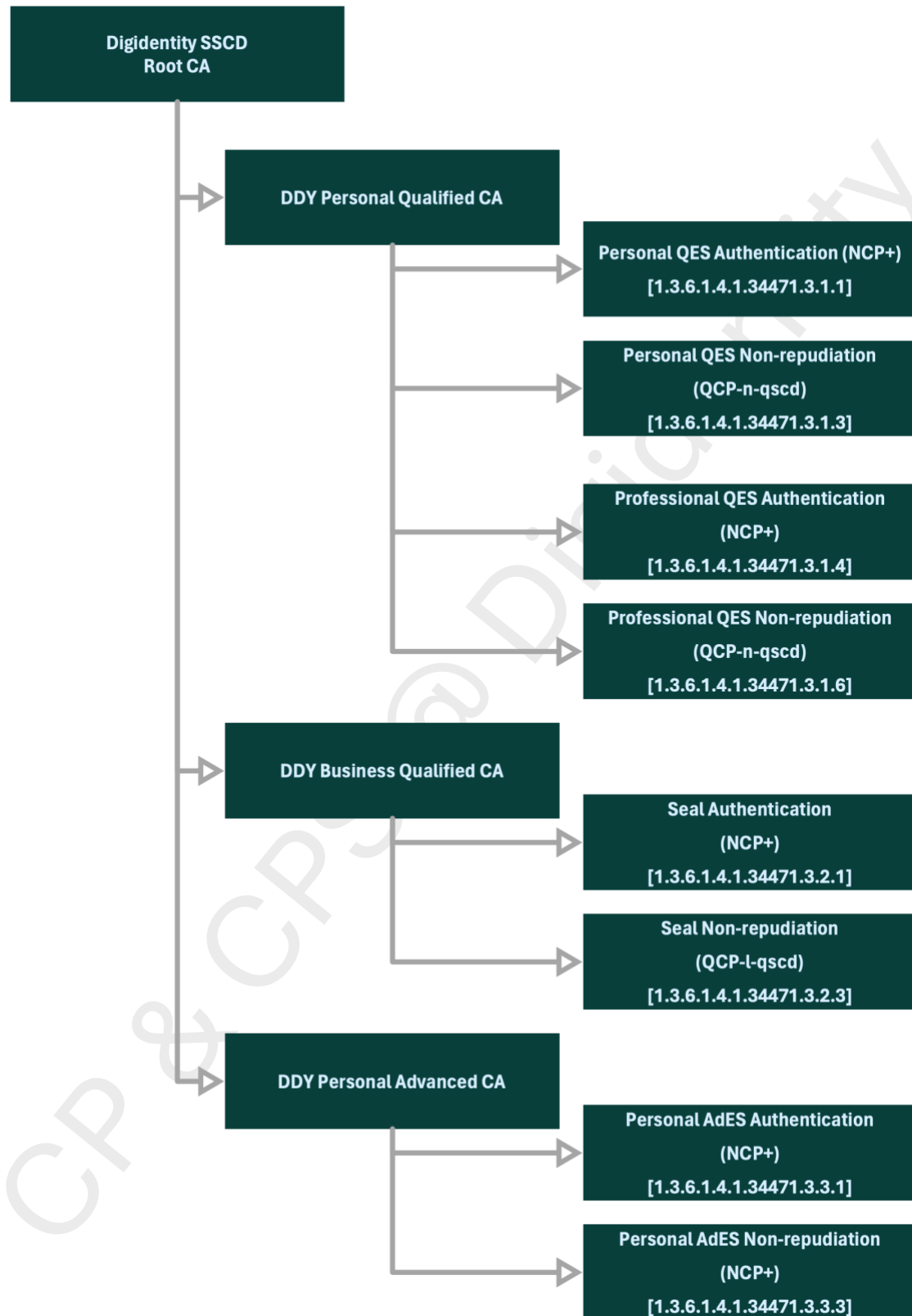
Figure 2 – Digidentity SSCD Root CA hierarchy
