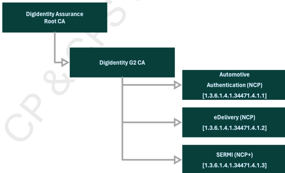
Figure 1 - Digidentity Assurance Root CA hierarchy
